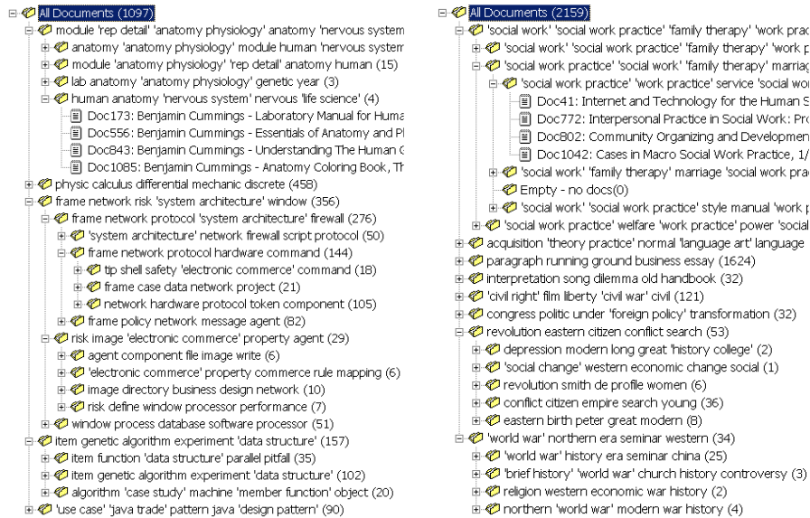
Fig. 1. Shows two trees of topics generated from Set B on the left and Set C on the Right, using the proposed method. The labels are chosen by ranking the top five terms with the lowest quantization error at each particular node. Multiple terms are marked with single quotes.
